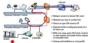
The cyber attack on the Ukraine is a sign of what is to come.
